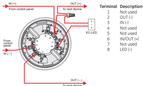
CRB4U-1 Detector relay base
