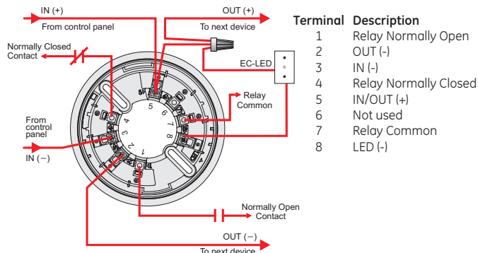
CRB4U-1 Detector relay base
