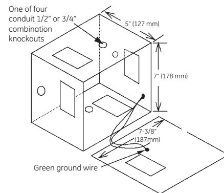
Knockout Locations
