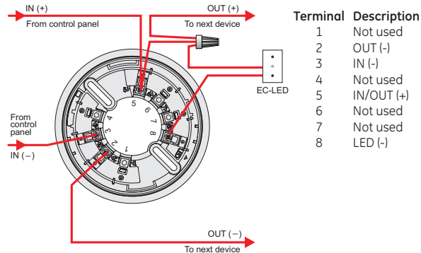
CSBU-3 Resistor base
