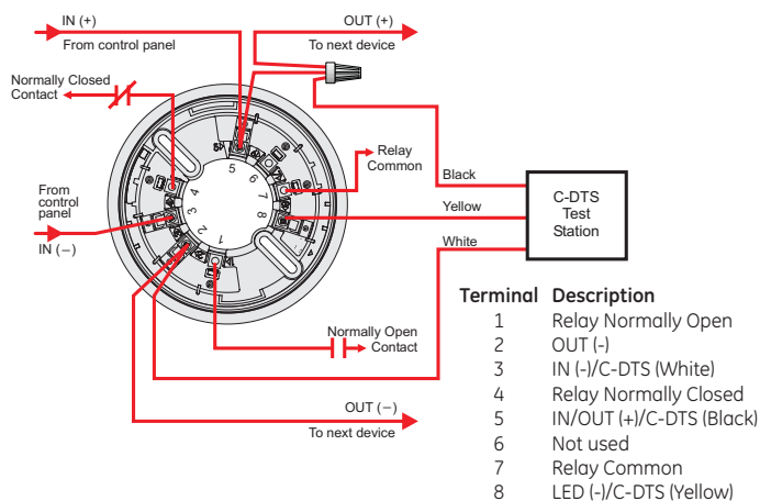
C-DTS Test Station
